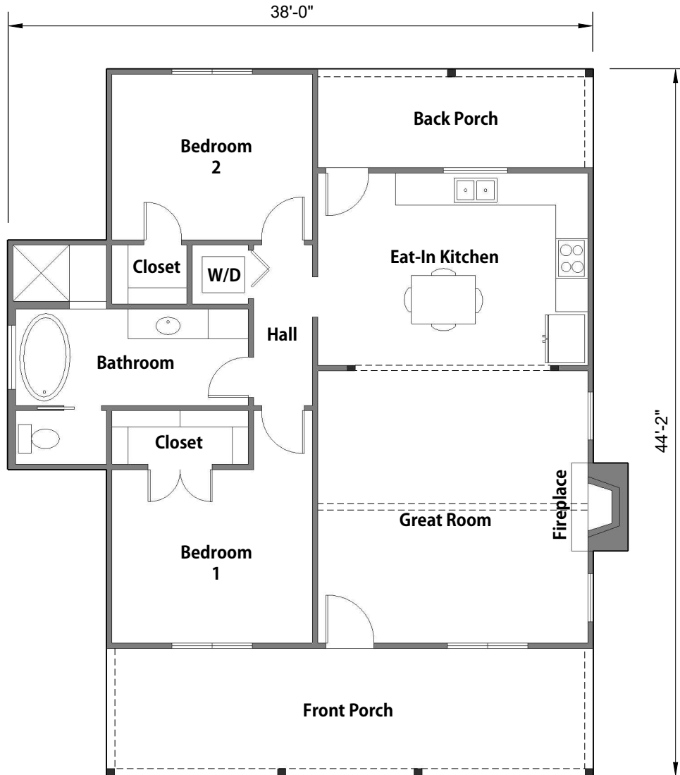
Floor Plan
