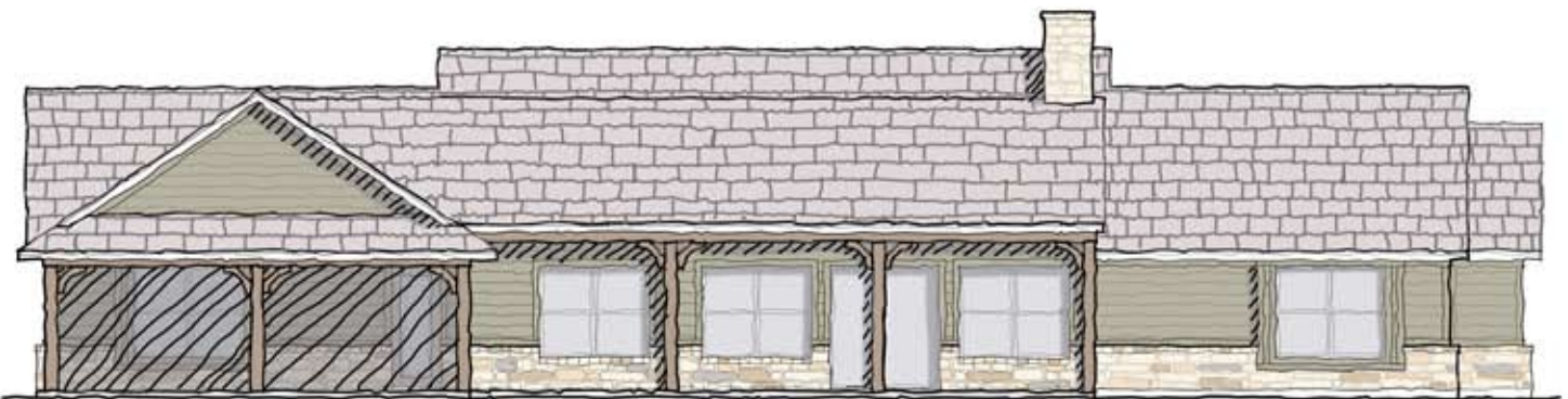
REAR ELEVATION
