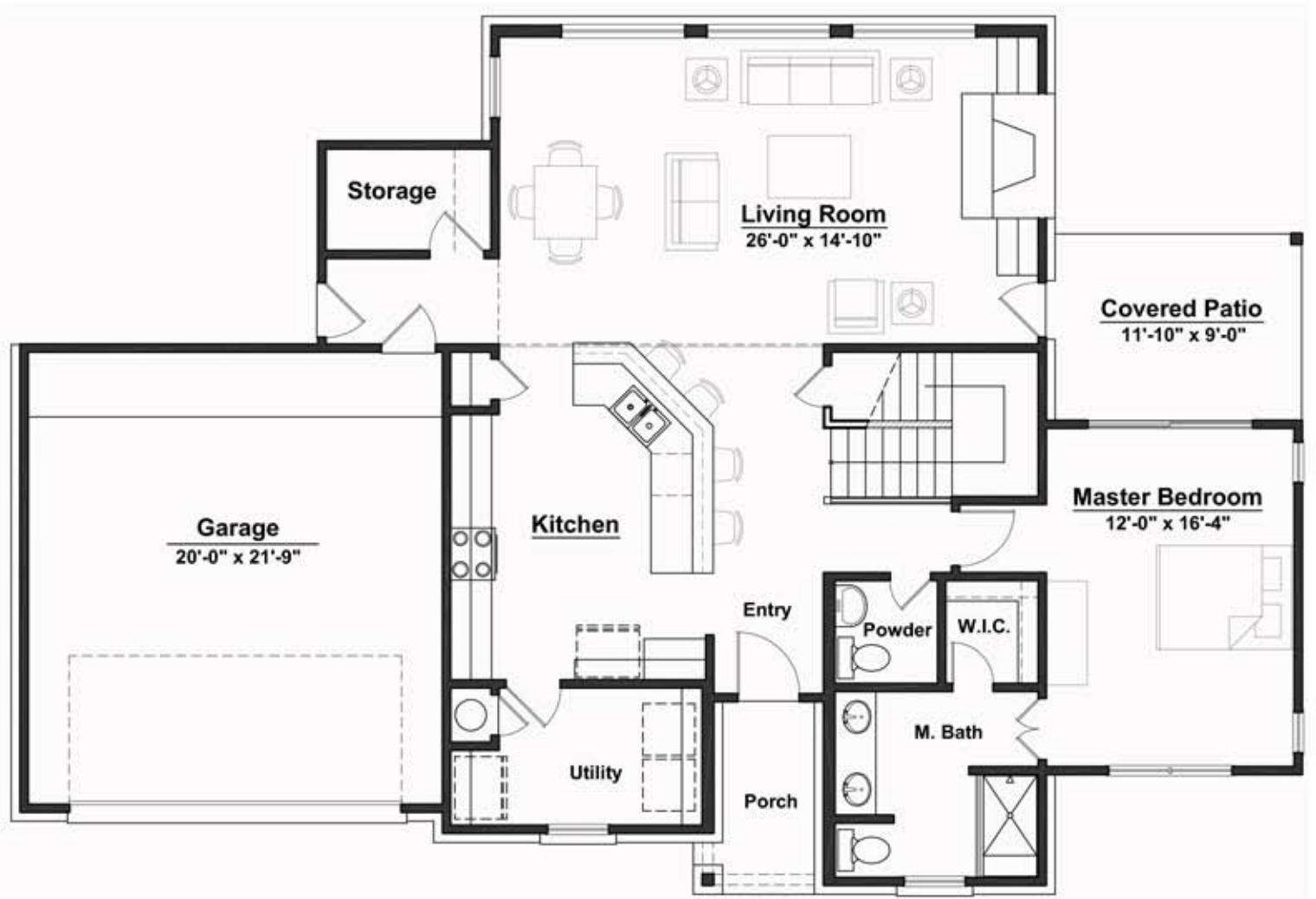
FIRST FLOOR PLAN @ GARAGE OPT.
