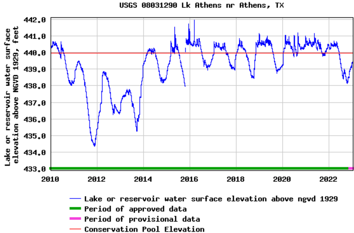
Figure 3. Water level for Lake Athens (2010-2022). Red line represents conservation pool level (440 ft. MSL).
